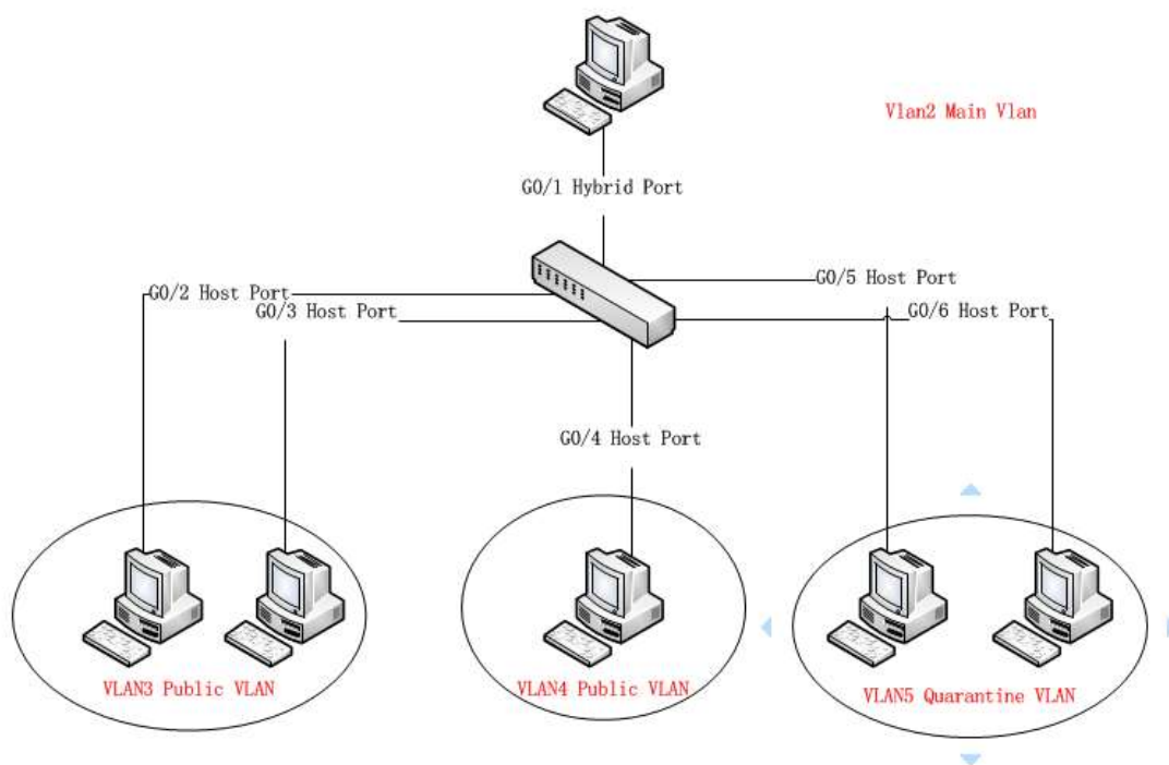
Figure 1: Typical Configuration of Private VLAN
